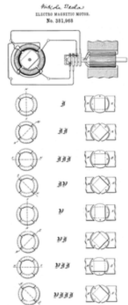
Drawing from U.S. Patent 381,968 ( https://patents.google.com/patent/US381968 ), illustrating the principle of Tesla's alternating current induction motor
