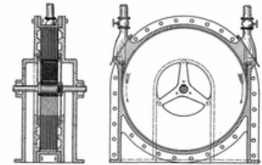
Tesla's bladeless turbine design
